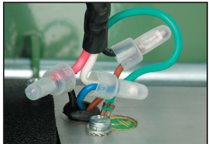
Figure 21. Motor connections.
